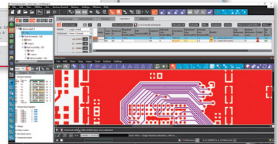
View and mark impedance lines
