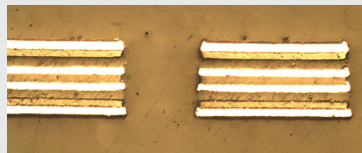
High quality through hole via in multi-layer flex
