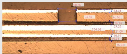
High quality blind via in multi-layer flex with adhesive
